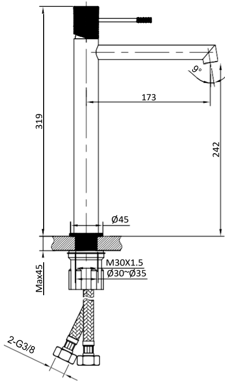
Installation drawing
